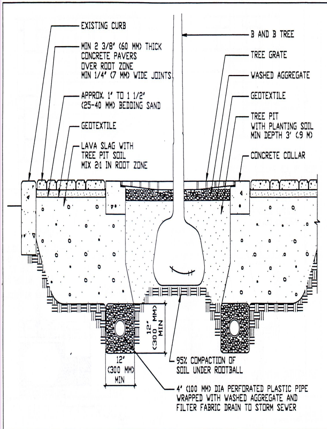
○ TREE PIT - NON-COMPACTED ROOT ZONE UNDER PAVERS
